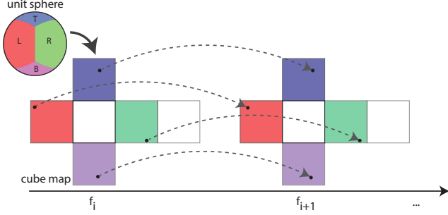
Figure 2: For each consecutive frame f_i and f_{i+1} , we map the unit spheres of the corresponding cameras to a cube map and perform feature tracking on each of the six image planes of the cube (T-top, B-bottom, L-left, R-right etc.) in parallel.
