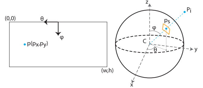
Figure 3: A 3D point P_i projects to the pixel p(p_x, p_y) in the (w \times h) panorama image and the point p_s(\cos\theta\sin\phi, \sin\theta\sin\phi, \cos\phi) on the unit sphere where \theta = 2\pi p_x/w and \phi = \pi p_y/h . When computing the matching cost of this point with neighboring views, we define a local patch around p_s on the unit sphere (in yellow) with axes directions (-\sin\theta, \cos\theta, 0) and (-\cos\theta\cos\phi, -\sin\theta\cos\phi, \sin\phi) .
